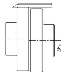
Radial/parallel displacement
