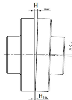
Angular displacement
