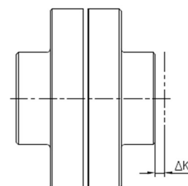
Axial displacement
